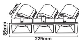
Dimension ( mm )
