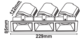
Dimension ( mm )
